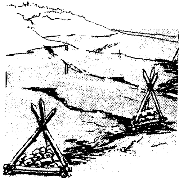
Figure 3-23. Timber tetrahedrons.
